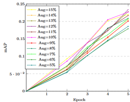
Figure 12. Initial value search with batch size 32. The data for the first six epochs is displayed, and each experiment is run three times.
