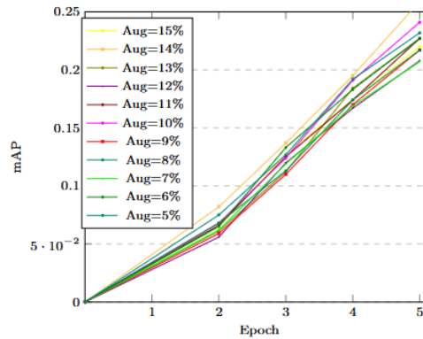
Figure 10. Initial value search with batch size 8. The data for the first six epochs is displayed, and each experiment is run three times.
