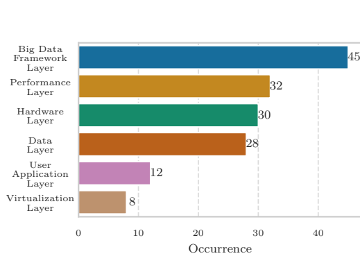
Fig. 3. Frequency analysis of parameter layers.
